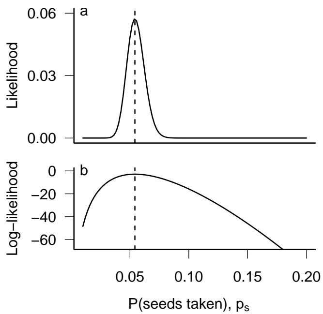
Figure 2: Likelihood and log-likelihood curves for predation probability p . Both curves have their maxima at the same point ( p = 0.054 ). Log-likelihoods are based on natural ( \log_e or \ln ) logarithms.
