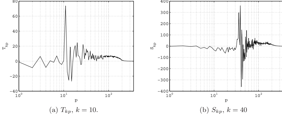
Figure 6: The time averaged energy ( T_{kp} ) and enstrophy ( S_{kp} ) transfer functions.
