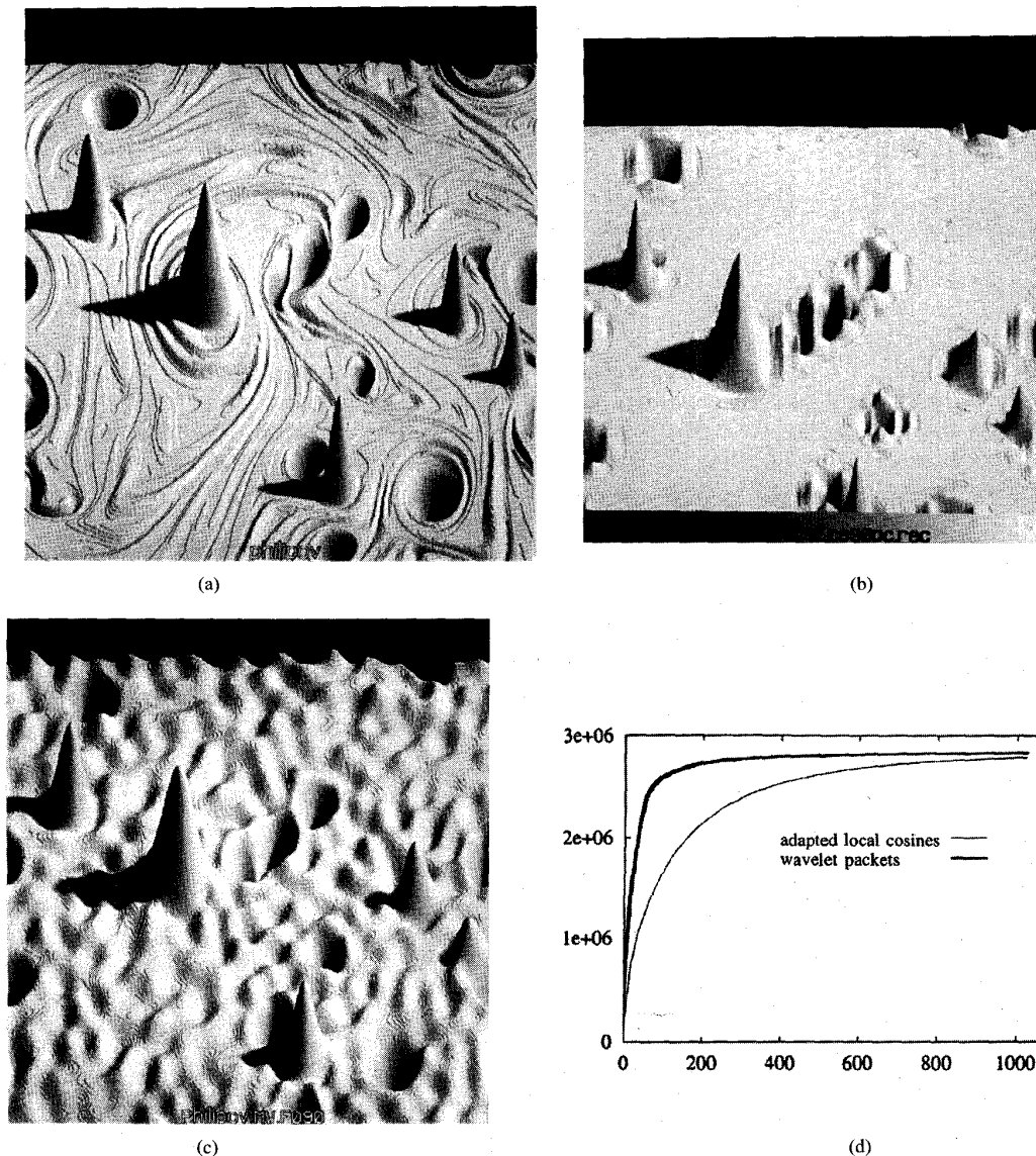
Fig. 4. Comparison between wavelet packet and adapted local cosine compression (this computation was done in collaboration with Echeide Cubillo). (a) The uncompressed vorticity field. (b) The vorticity field reconstructed from the 70 strongest wavelet packet coefficients, which contain 90% of the enstrophy. (c) The vorticity field reconstructed from the 425 strongest adapted local cosine coefficients, which contain 90% of the total enstrophy. (d) Enstrophy contained in the retained coefficients versus their number. We observe, for instance, that 70 wavelet packet coefficients retain 90% of the total enstrophy, while 70 adapted local cosine coefficients retain only 50% of the total enstrophy.
