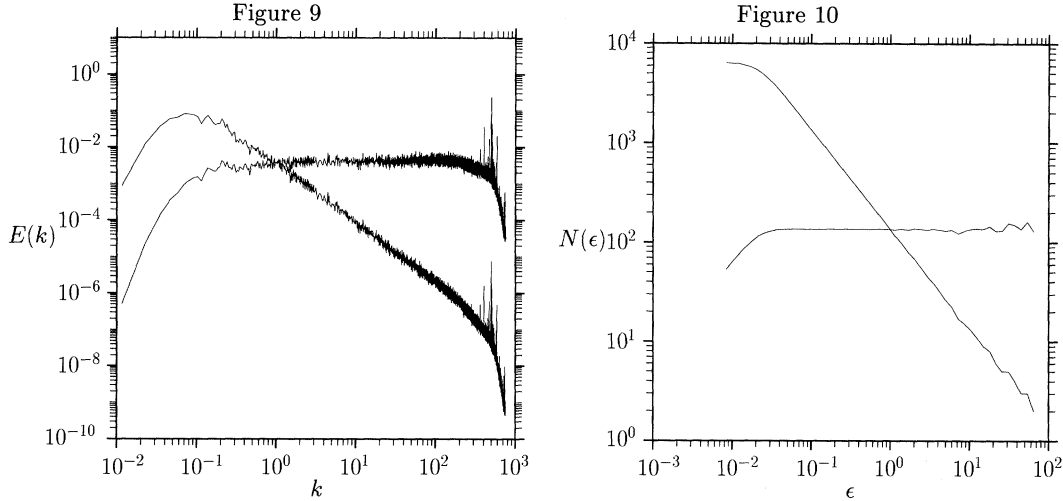
Figure 9. Energy spectrum of the longitudinal velocity component of experimental turbulence (the Taylor hypothesis has been used). Horizontal curve is \propto k^{5/3} . The large scale part of the spectrum is \sim k^4 ( k < 0.04 \text{ m}^{-1} ). The integral scale is at about k = 7.18 \text{ m}^{-1} , the Taylor microscale is at k = 175 \text{ m}^{-1} and the Kolmogorov scale (not resolved) is at k = 18000 \text{ m}^{-1} . The data have been divided into 32 131072 point segments and the Parzen window has been used.
