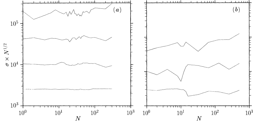
Figure 12. (a) \sigma_w(a) \times N^{\frac{1}{2}} of a random phase signal as a function of number of realizations at scales a = 1.94 \times 10^{-2} , 0.106, 0.575, 3.13 (from bottom). (b) \sigma_w(a) \times N^{\frac{1}{2}} of a Weierstrass function ( f(x) = \sum_{k=1}^{\infty} \lambda^{(s-2)k} \sin(\lambda^k t) , \lambda = 1.5 , s = 1.5 , the series is truncated after the first 50 terms) as a function of number of realizations at scales a = 1.14 \times 10^{-3} , 6.20 \times 10^{-3} , 0.0337 (from bottom).
