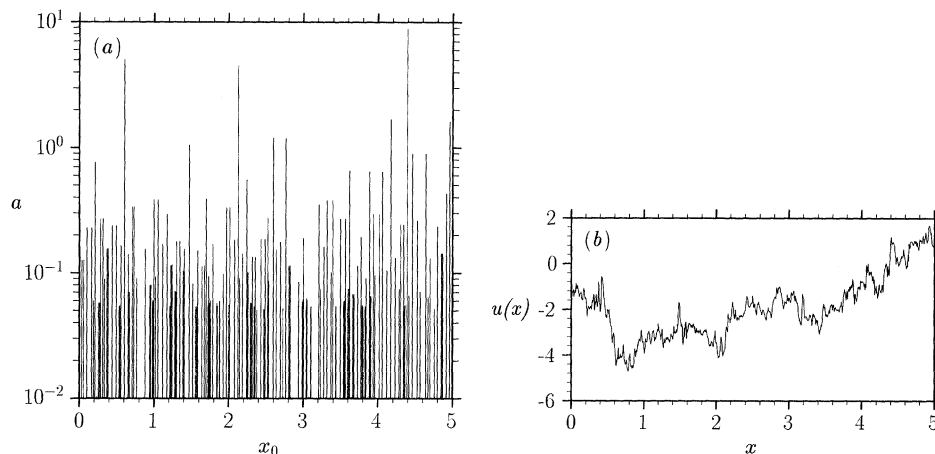
Figure 2. (a) Straightened zero crossings of the Mexican hat wavelet transform of a 1200 point long segment of the longitudinal component of an experimental turbulent velocity signal. (b) Original signal.
