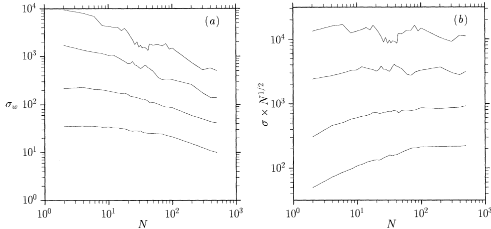
Figure 14. (a) \sigma_w(a) at scales a = 1.94 \times 10^{-2} , 0.106, 0.575, 3.13 for the 'spiral' function \sin(x^{-\frac{1}{2}}) . (b) Same as (a), but \times N^{\frac{1}{2}} . Note how \sigma_w(a) remains approximately constant at small scales and moderate N , and becomes more like a random phase signal (decreasing like N^{-\frac{1}{2}} ) at large scales and large N .
