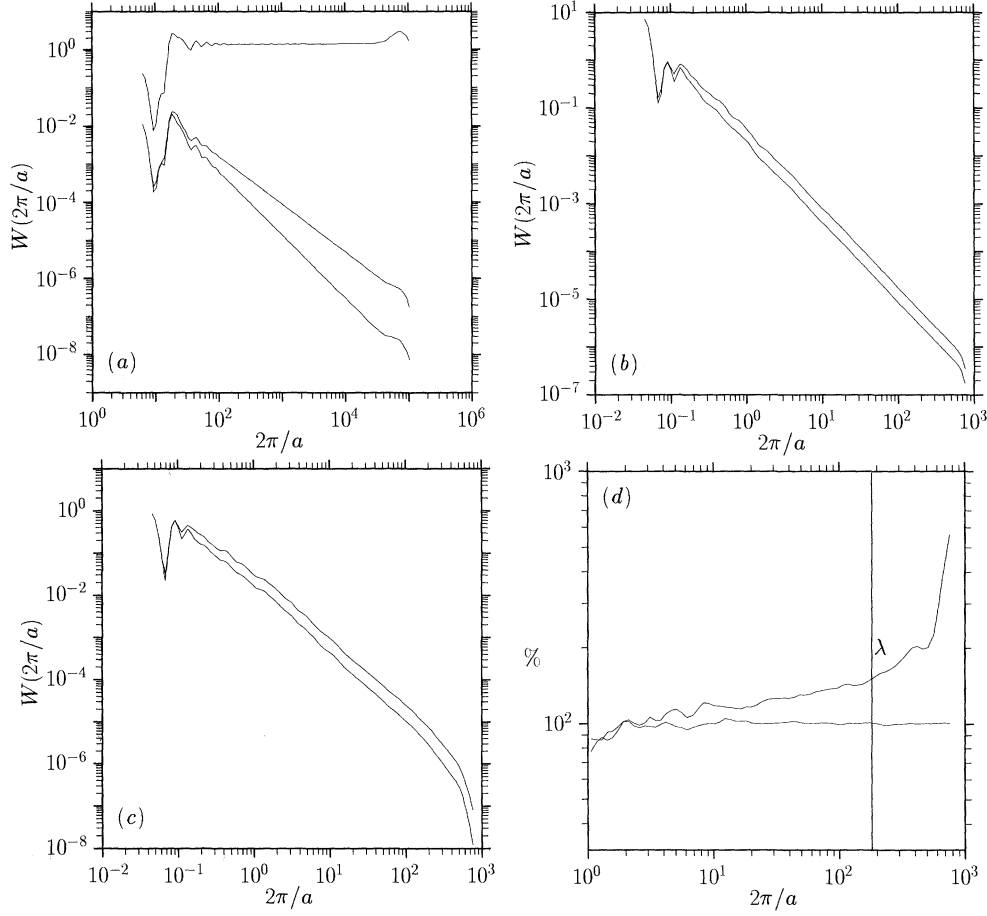
Figure 18. Spatial fluctuation of wavelet energy (average of 50 realizations). (a) \sin(t^{-1/2}) spiral. Lower curve is wavelet energy spectrum, middle curve is plus one standard deviation and upper curve is the wavelet spectrum \times a^{-5/3} . (b) Random phase signal ( E(k) \propto k^{-5/3} ). Lower curve is wavelet energy spectrum, upper curve is plus one standard deviation. (c) Experimental turbulence data. Lower curve is wavelet energy spectrum, upper curve is plus one standard deviation. (d) Percent standard deviation of wavelet energy spectrum ( I(a) ). Top curve is the experimental turbulence data, lower curve is the random phase signal, \lambda indicates the Taylor microscale.
