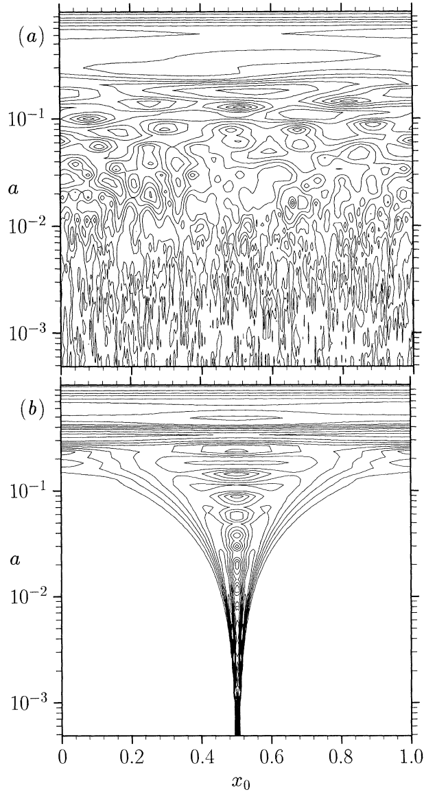
Figure 11. (a) Morlet wavelet transform of a random phase signal with energy spectrum E(k) \propto k^{-5/3} . (b) Morlet wavelet transform of \sin(2\pi x^{-1/2}) ( E(k) \propto k^{-5/3} ).
