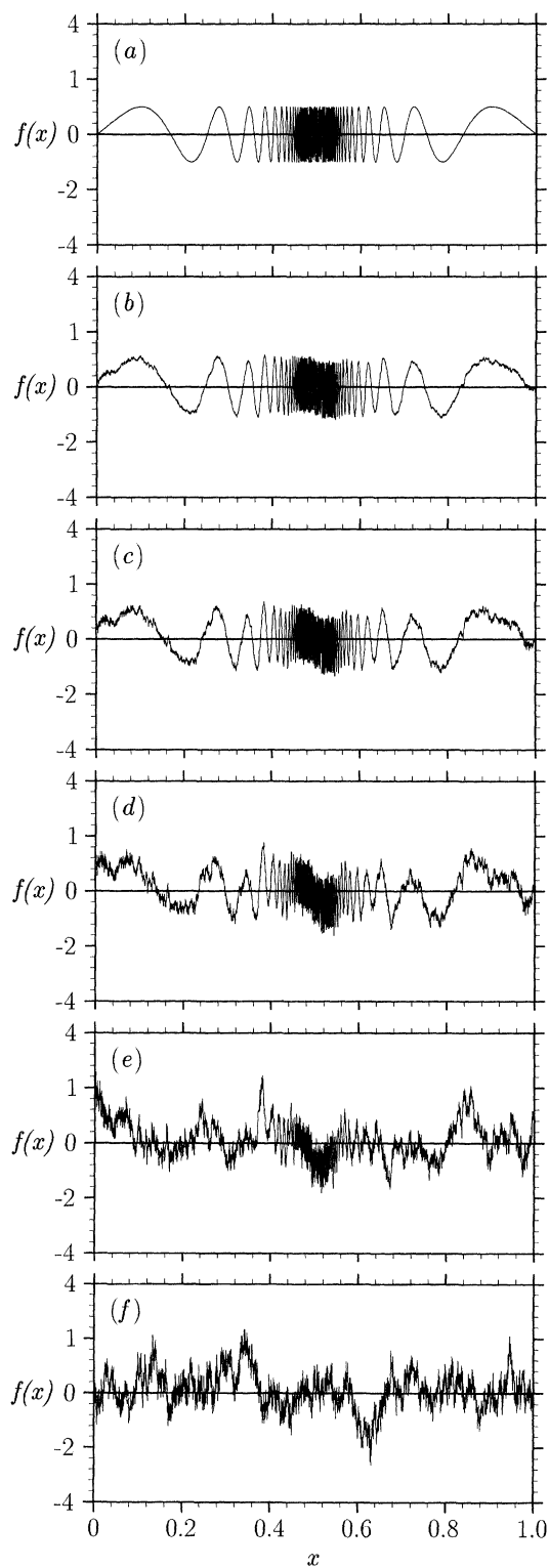
Figure 6. \sin 2\pi/x accumulating function with increasing levels of phase noise. (a) 0% noise.
