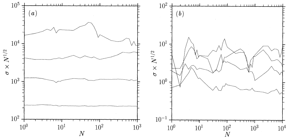
Figure 17. \sigma_w(a) \times N^{1/2} as a function of number of realizations. (a) 4096pt (17.0 m) long segments (scales 1.94 \times 10^{-2} , 0.106, 0.575, 3.13 m). (b) \sigma_w(a) \times N^{1/2} for 32pt (0.133 m) long segments (scales 1.10 \times 10^{-2} , 2.03 \times 10^{-2} , 3.76 \times 10^{-2} , 6.96 \times 10^{-2} ). Note the deviation from the H-fractal N^{-1/2} slope for N < 10 .
