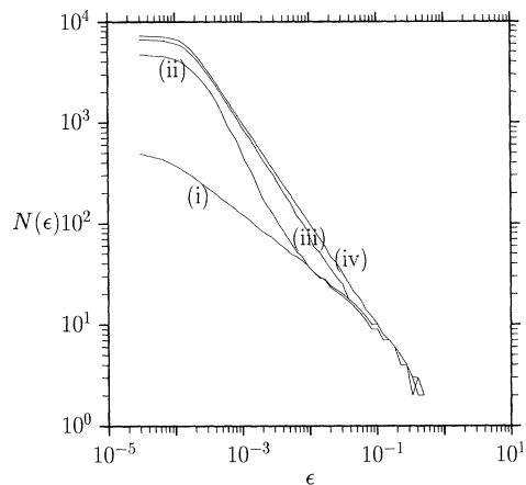
Figure 7. Eddy capacity curves for a \sin 2\pi/x eddy with phase noise levels of (i) 0%, (ii) 0.1%, (iii) 1% and (iv) 50%. With a noise level of 1% the ‘eddies’ are essentially space filling, D_E = 1 .
