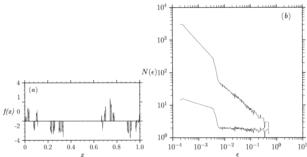
Figure 8. (a) Random phase k^{-5/3} signal multiplied by a middle-third Cantor set. (b) Eddy capacity curve for the signal in (a). The lower curve is \epsilon^{\log 2 / \log 3} N_E(\epsilon) and shows that, at the larger scales \epsilon , D_E is equal to D_K of the Cantor set filter. Here D_K = \log 2 / \log 3 .
