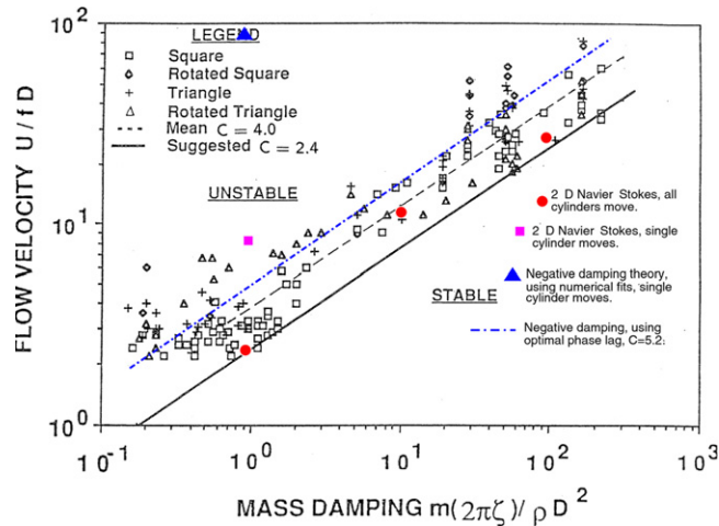
Fig. 5. Potential flow and 2-D Navier–Stokes calculations compared with data and theory. Results are normalized with respect to the gap velocity U_g . (Modified from Blevins' (2001) Figs. 5 and 6.)
