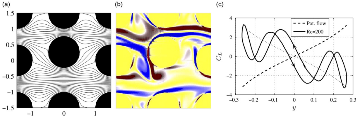
Fig. 3. Flow induced vibration in an inline tube array with P/D=1.5 . The central cylinder is free to move in the transverse direction only. (a) Potential flow streamlines. (b) Re=200 vorticity (red is positive, blue is negative). (c) Comparison of lift force (normalized by U_g ) as a function of cylinder position for potential flow and Navier–Stokes flow at Re=200 . The lift force for the Navier–Stokes flow has been averaged over many periods of cylinder oscillation. The dotted line is -C_L(y) for the potential flow and the arrows give the direction of cylinder motion (note hysteresis). (For interpretation of the references to color in this figure legend, the reader is referred to the web version of this article.)
