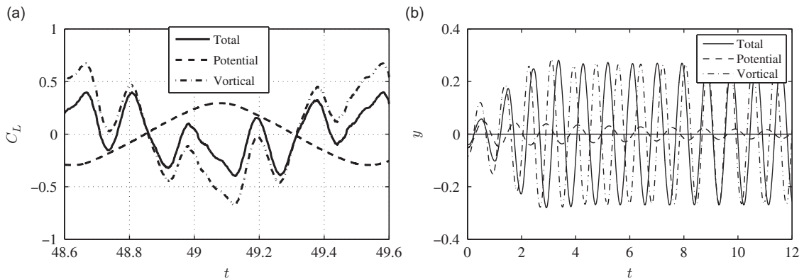
Fig. 6. The 2-D Navier–Stokes simulation results for a 3 \times 3 periodic array with the central cylinder free to move in the transverse direction only and a mass damping of one. (a) Total lift compared with its potential and vortical parts. (b) Cylinder amplitude when cylinder is forced by the total force, only the potential force, or only the vortical force.
