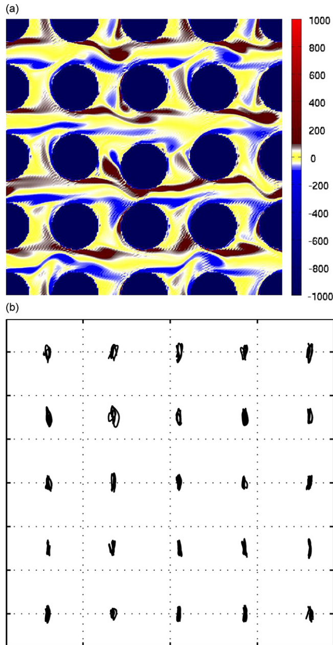
Fig. 4. (a) Vorticity field at Re=200 for a 5 \times 5 periodic unit cell with the central cylinder free to move in the transverse direction. (b) Cylinder trajectories for a 5 \times 5 periodic unit cell with all cylinders free to move.
