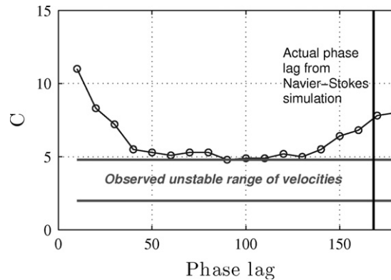
Fig. 2. Nonlinear stability calculations for periodic potential flow with 2 \times 2 unit cell. The potential flow value of the critical velocity coefficient C is close to the experimental data for a wide range of phase lags.
