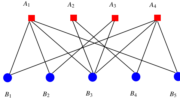
Fig. 2.4 A bipartite graph with 5 banks (blue nodes) co-owning 4 assets (red nodes).
