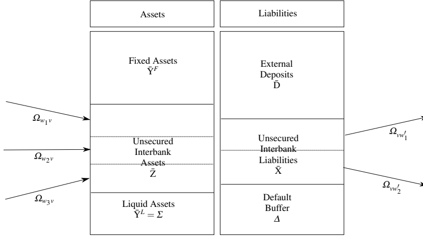
Fig. 2.2 The stylized balance sheet of a bank v with in-degree j_v = 3 and out-degree k_v = 2 . Banks w_1, w_2, w_3 are debtors of v while w'_1, w'_2 are its creditors.
