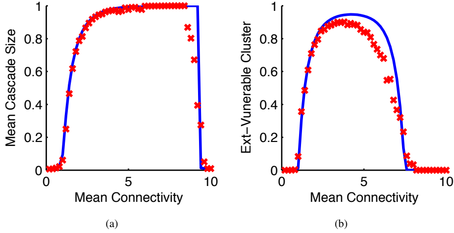
Fig. 5.1 These two graphs show (a) the mean fractional cascade size, and (b), the fractional extended vulnerable cluster size, in the benchmark Gai-Kapadia model as a function of mean degree z , as computed using the large N analytics of Theorem 11 (blue curve) and by Monte Carlo simulation (red crosses). In Figure (a), the Monte Carlo computation involved N_{\text{sim}} = 50 realizations of the N = 10000 node graph, each with an initial seed generated by selecting nodes independently with probability 0.5%. In Figure (b), the simulation involved N_{\text{sim}} = 2500 realizations of the N = 10000 node graph and a single random initial seed node.
