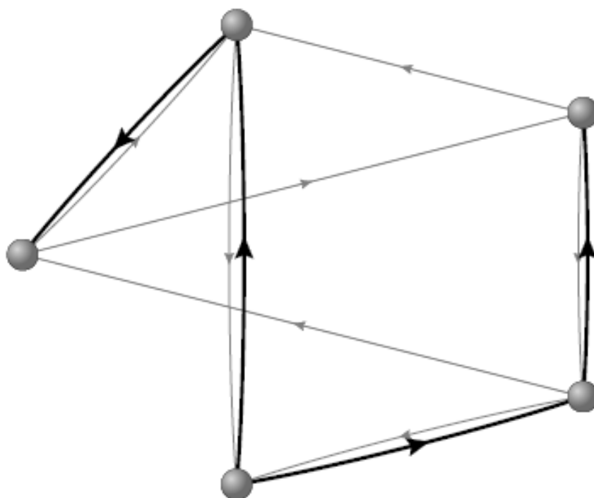
Chart 1: A weighted, directed network with five nodes
