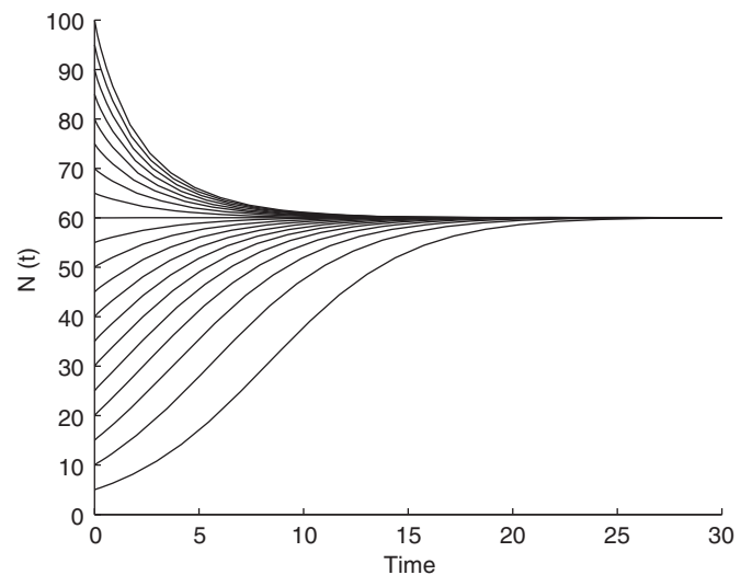
Fig. 2. N(t) versus time, for constant initial data \phi(s) \equiv \phi on [-\tau, 0] increased from 5 to 100 by steps of 5. Parameter values are \gamma = 1, \mu = 0.5, \kappa = 0.005 , and \tau = 0.29 , resulting in \bar{N} \simeq 60 . This graph is almost indistinguishable from the graph that would be found by solving (1) using K = 60 and r = 0.3 .
