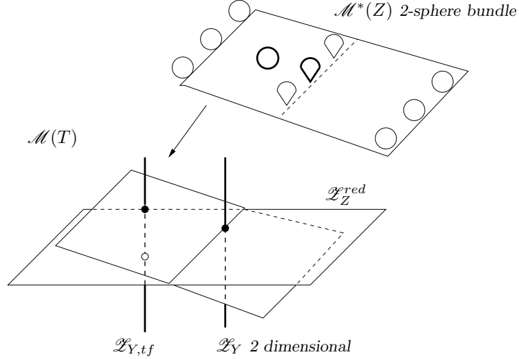
FIGURE 3. The effect of a twisting perturbation on a pointed 2-sphere. Here \mathcal{M}^*(Z) is 4-dimensional and the map \zeta_Z^*: \mathcal{M}^*(Z) \rightarrow \mathcal{M}(T) has 2-sphere fibers.
