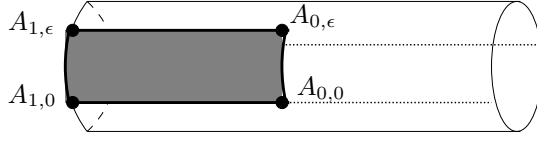
FIGURE 4. The family A_{s,t} is the shaded rectangle within a cylindrical component of R^{red}(Z, SU(3)) .
