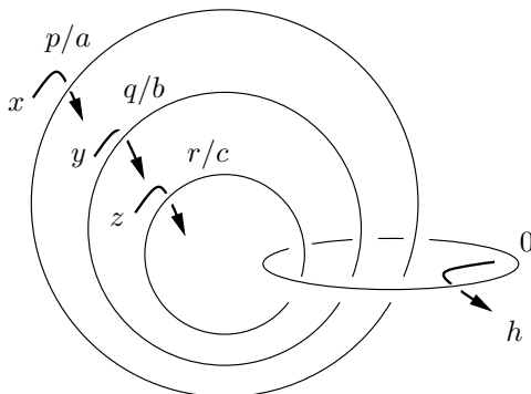
FIGURE 1. A surgery description of the Brieskorn manifold \Sigma(p, q, r) indicating the Wirtinger generators x, y, z , and h for \pi_1(\Sigma) .
