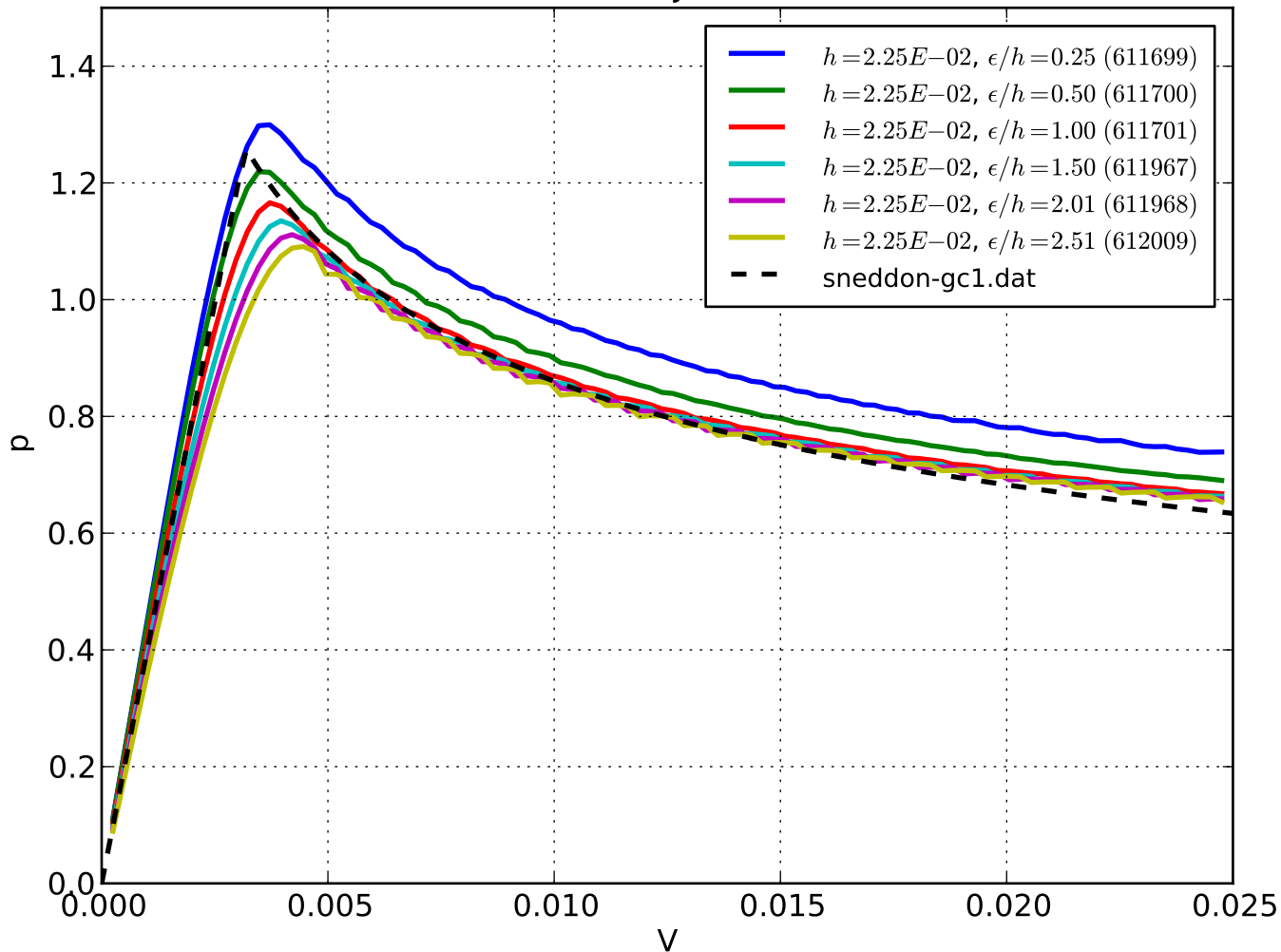
Pressure vs. injected volume
